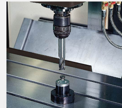
AUTOMATIC TOOL LENGTH MEASURING DEVICE (DAHLI)
