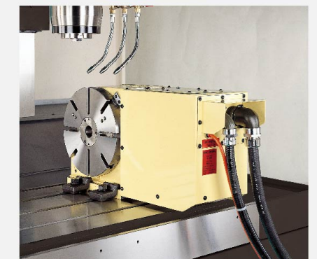
4TH AXIS CONTROL AND ROTARY TABLE
